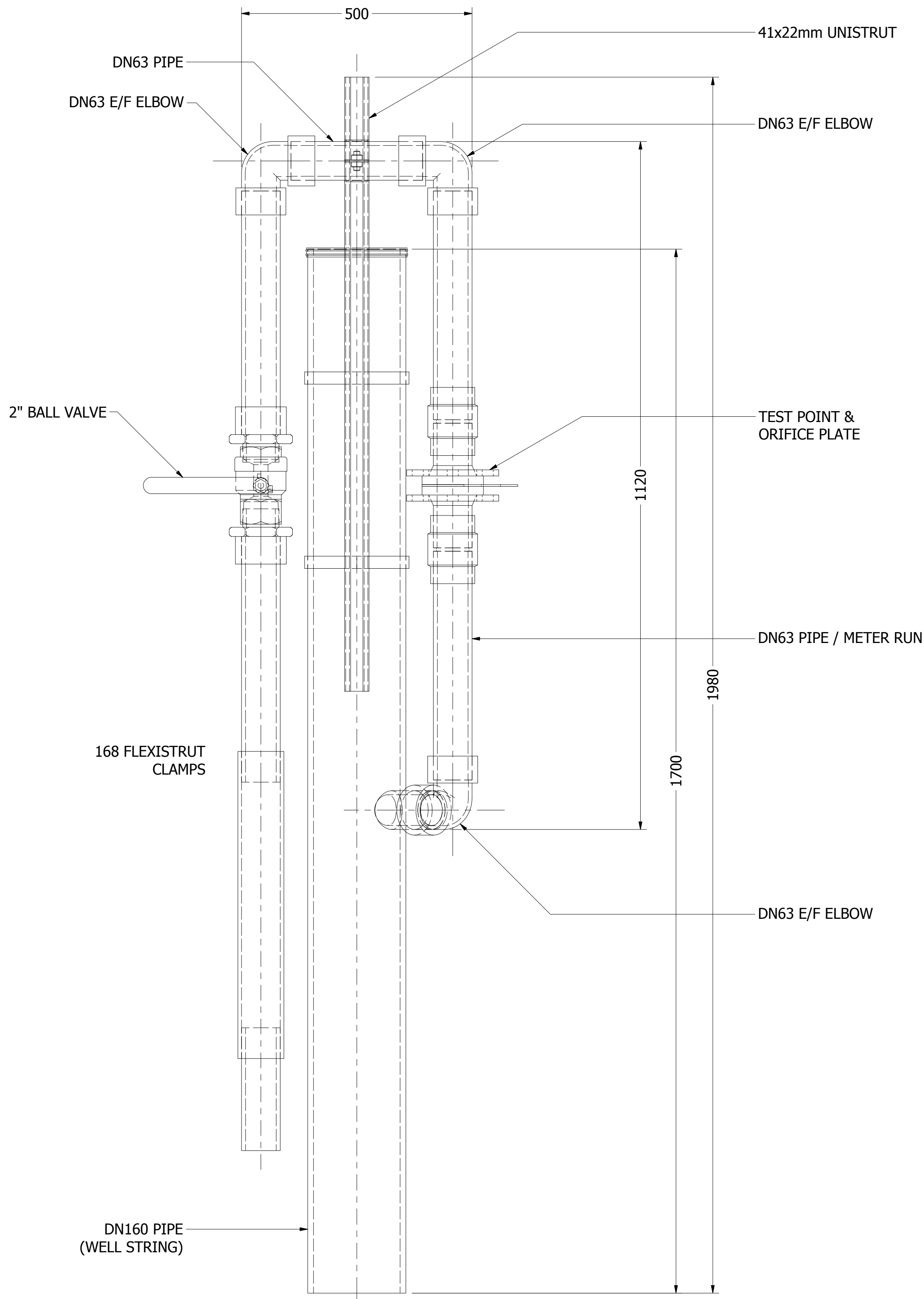
STANDALONE WELL ASSEMBLY SCALE (DNS)
